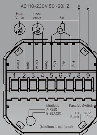
Four Pipe, On/off
